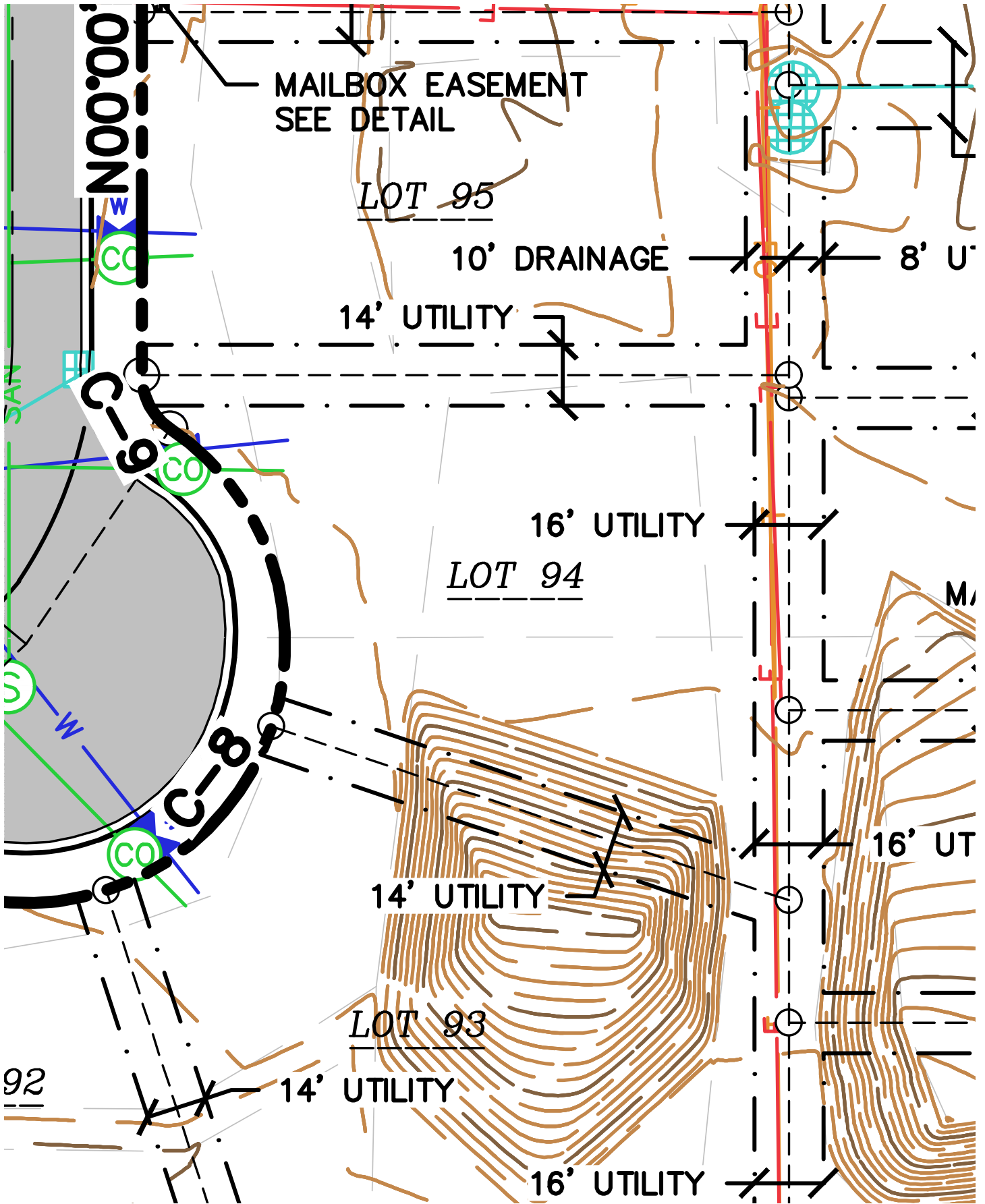
Lot 94 | Existing Conditions
