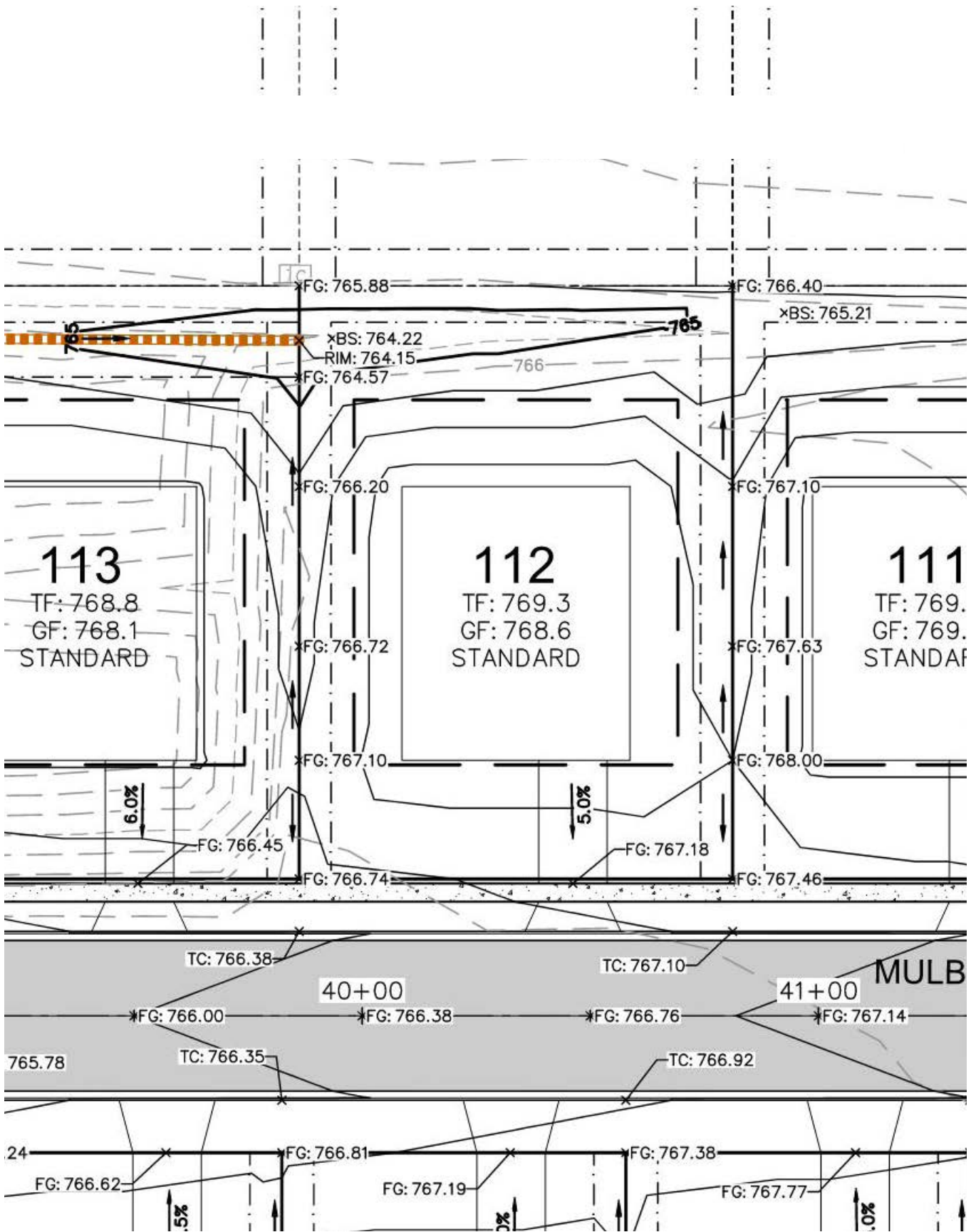
Lot 112 | Grading Parameters
