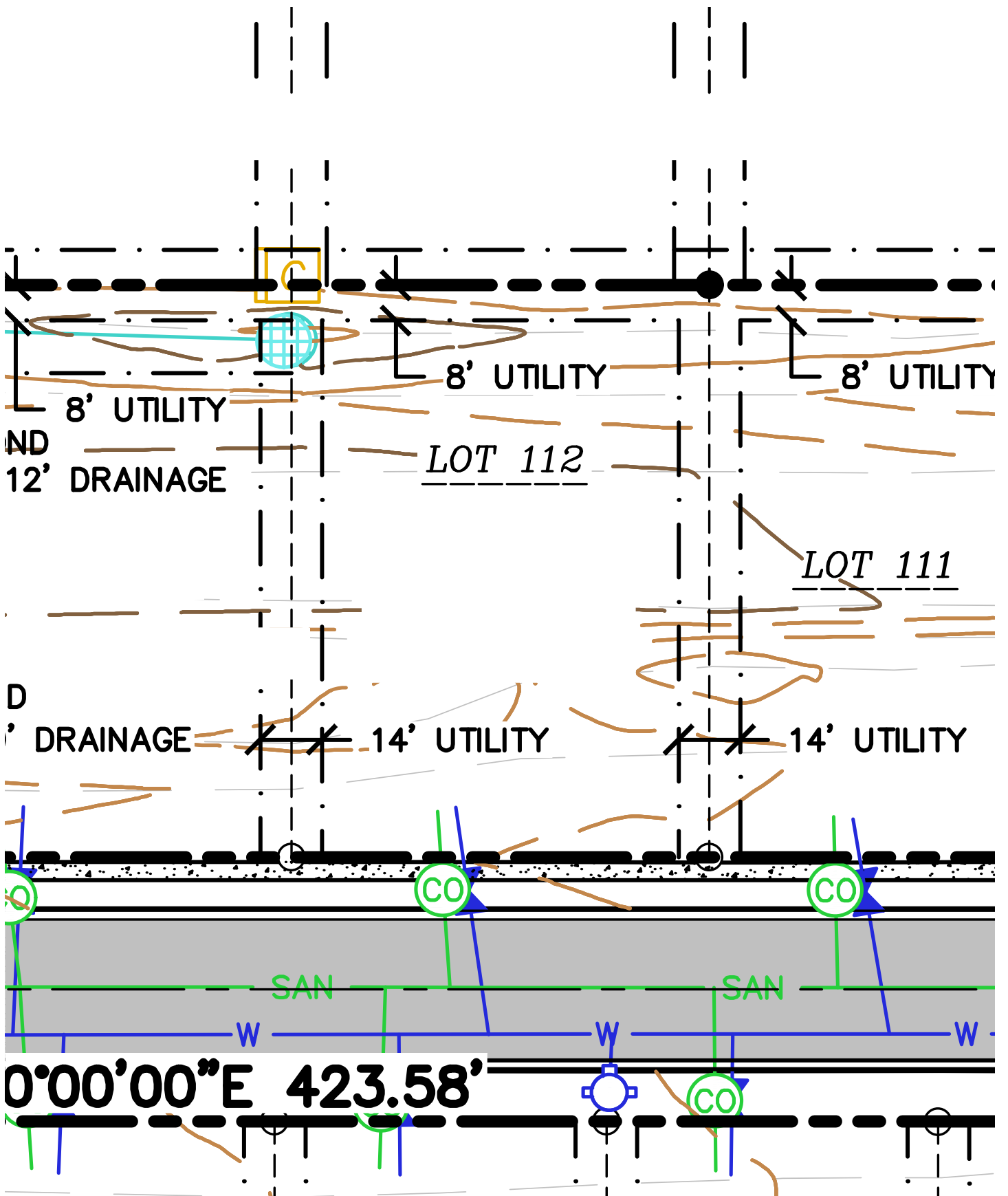
Lot 112 | Existing Conditions
