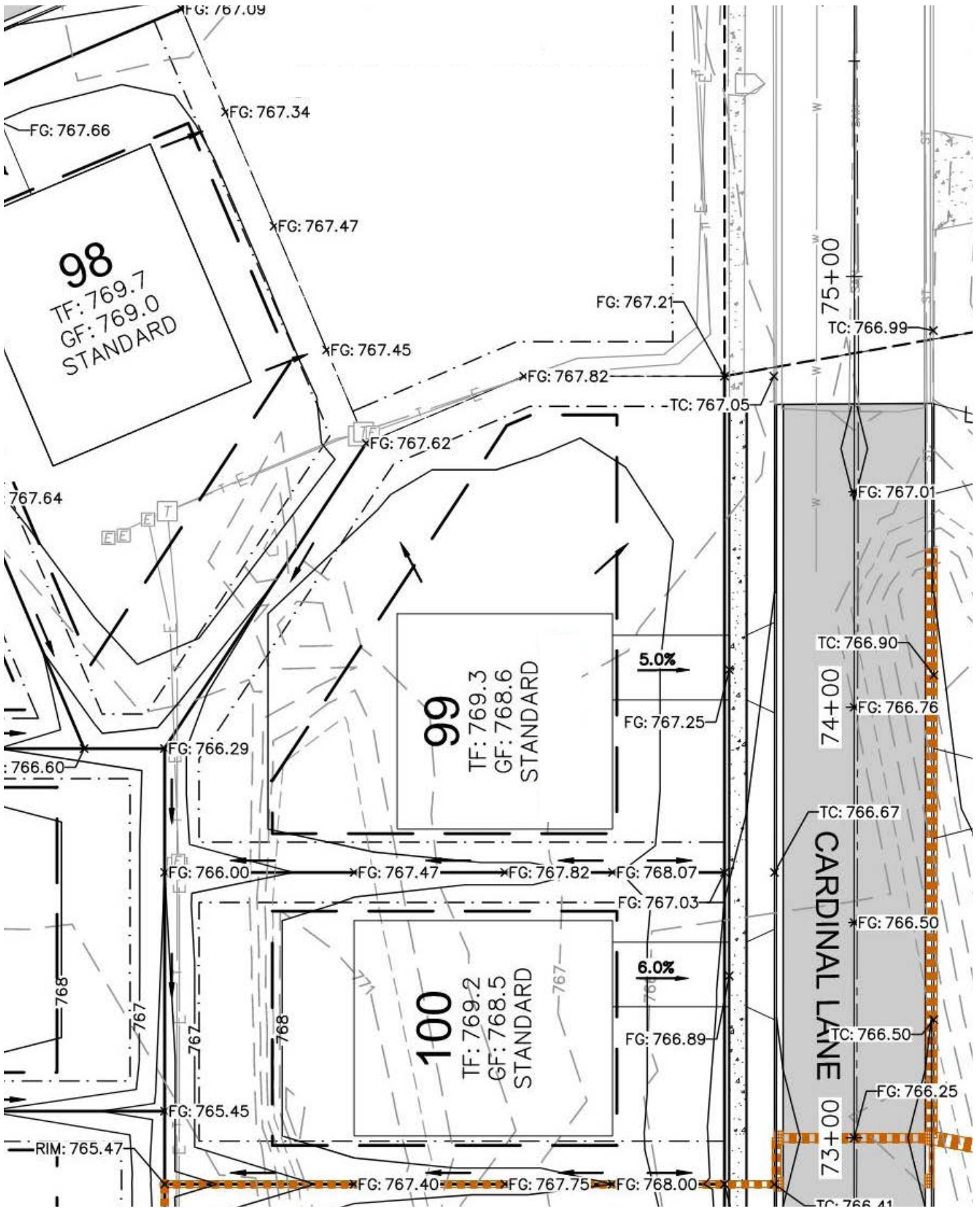
Lot 99 | Grading Parameters
