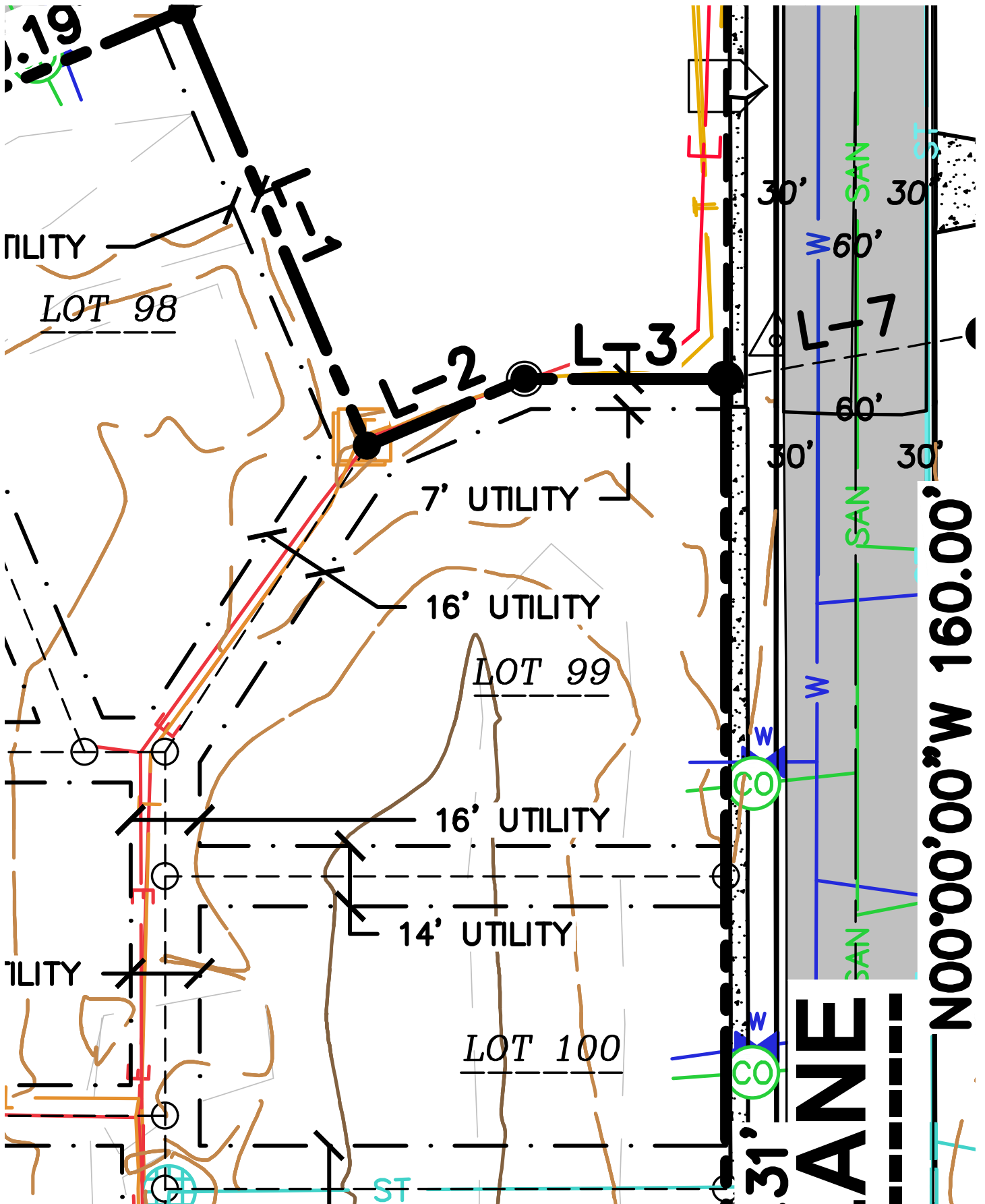
Lot 99 | Existing Conditions
