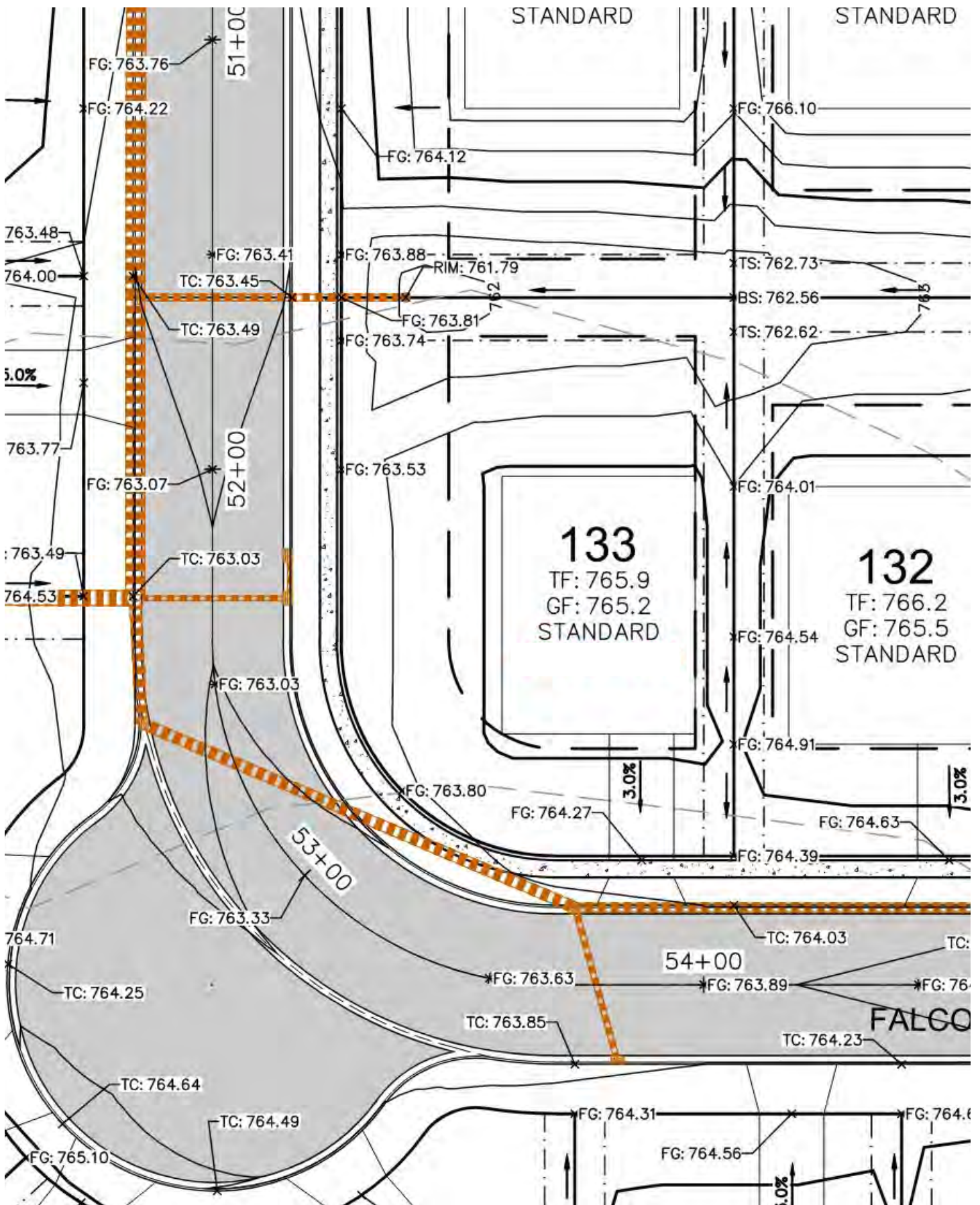
Lot 133 | Grading Parameters
