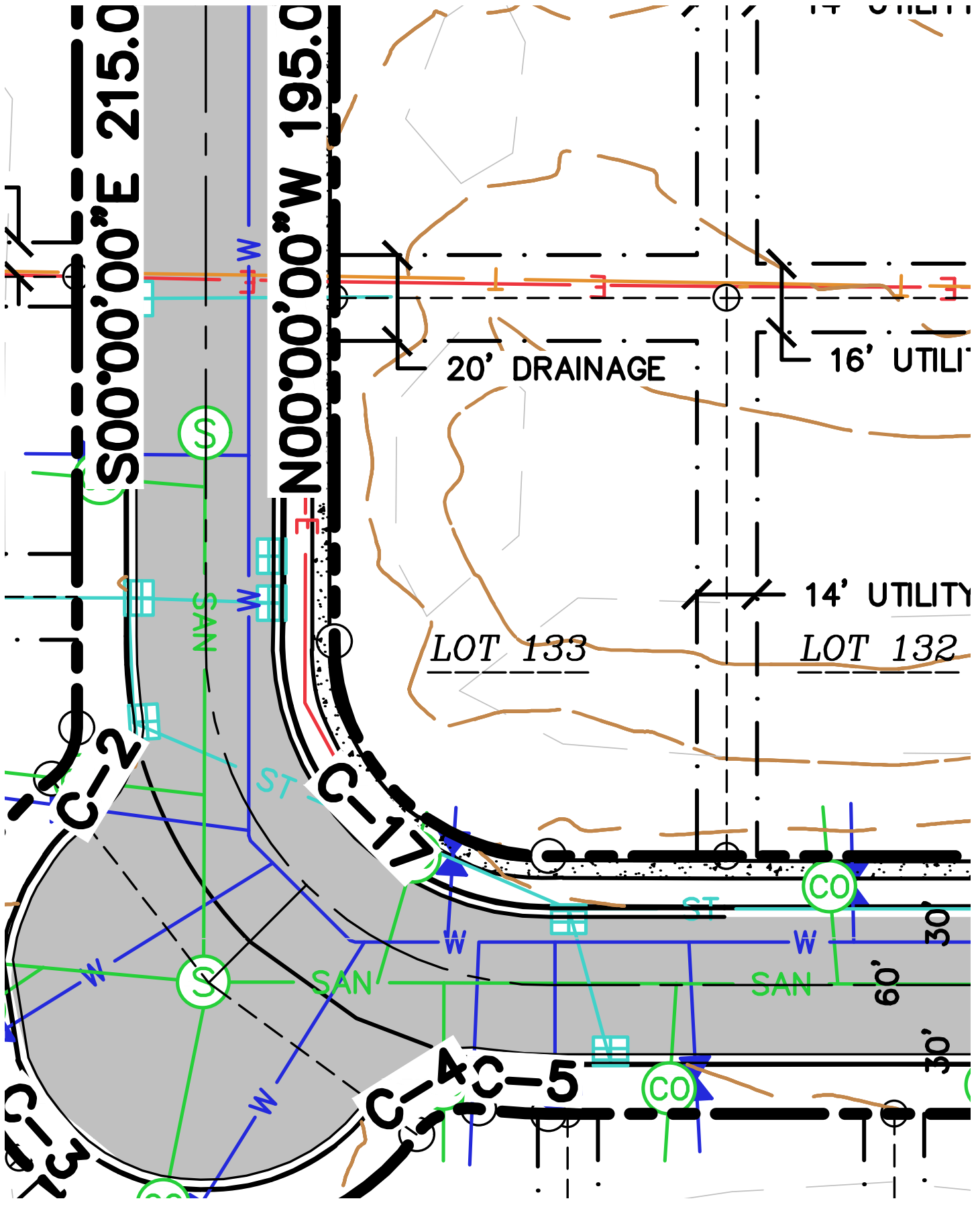
Lot 133 | Existing Conditions
