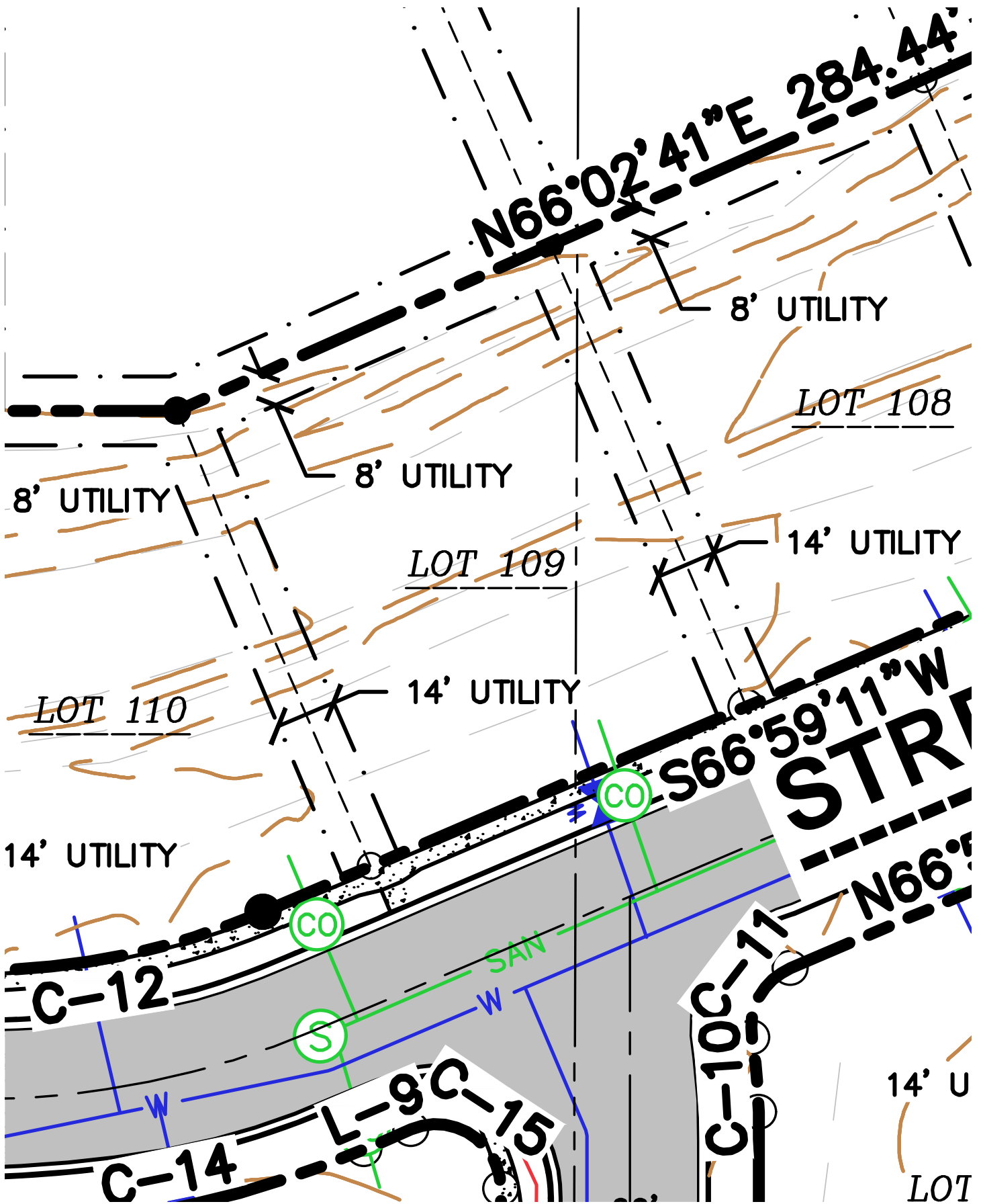
Lot 109 | Existing Conditions
