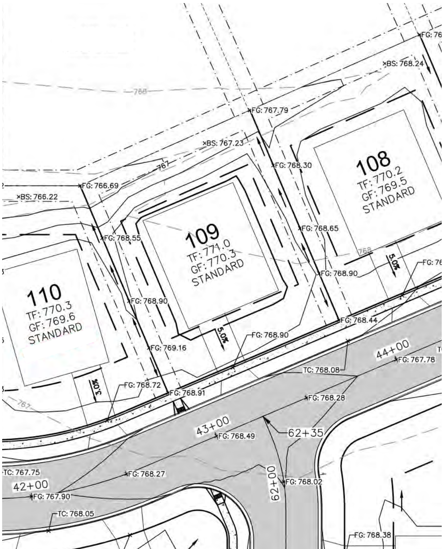
Lot 109 | Grading Parameters
