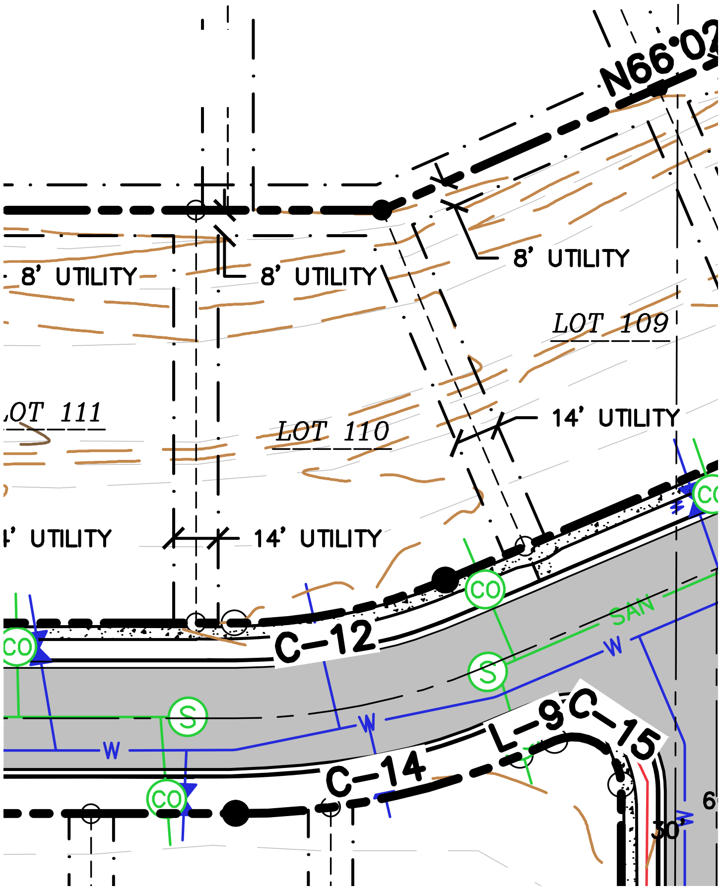
Lot 110 | Existing Conditions
