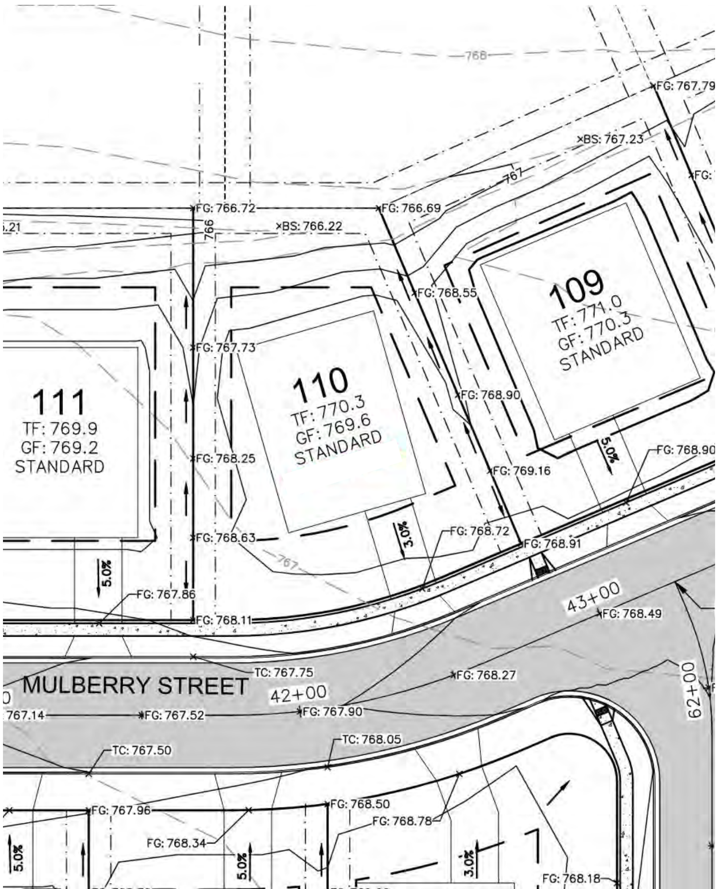
Lot 110 | Grading Parameters
